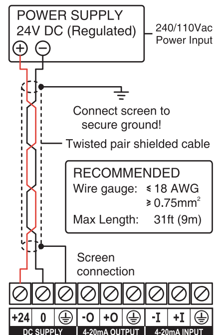
Figure 1: Electrical connection terminal (Located under the terminal cover)
